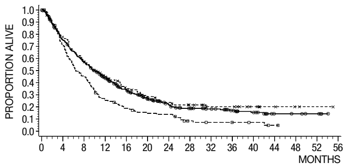
Figure 1: Overall Survival
