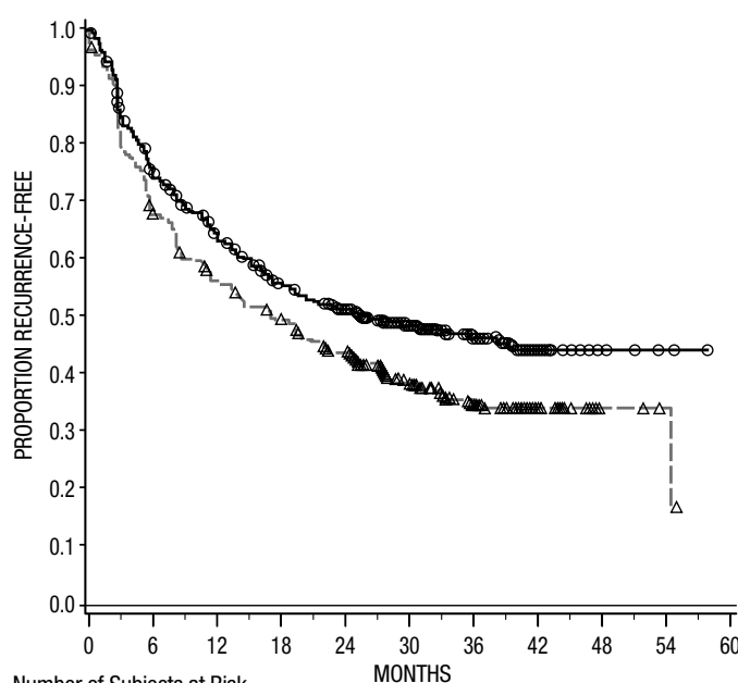
Figure 2: Recurrence-Free Survival
